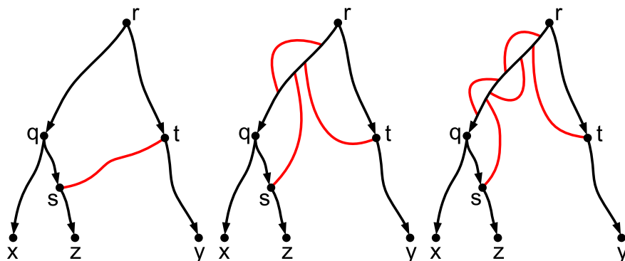
Figure 4.30: Several examples of twist covers (the red, undirected paths) from the proof of Lemma 4.18. Note that these exhibit the regular, interleaved structure associated with minimum-length twist covers.
