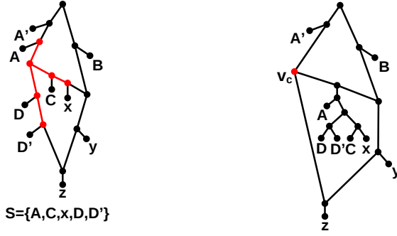
Figure 4.19: Construction of N' (on the right) if N (on the left) is of type 2a with all leaves on sides C and D and some on side A in S .
