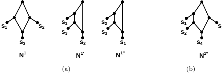
Figure 4.9: (a) The three networks N^1, N^{1'} and N^{1''} that are consistent with T^1 = \{s_1 s_3 | s_2, s_2 s_3 | s_1\} and (b) network N^{1*} , which is the unique network that is consistent with the set of triplets consistent with N^{1*} .
