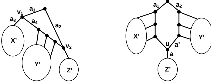
(a) Skew cycle; the second case in Lemma 4.10. (b) Non-skew cycle; the third case in Lemma 4.10.
