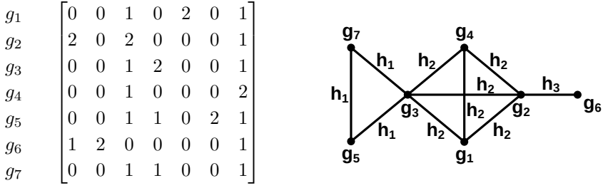
Figure 3.1: Example of a genotype matrix with corresponding compatibility graph, with h_1 = (0, 0, 1, 1, 0, 0, 1) , h_2 = (0, 0, 1, 0, 0, 0, 1) and h_3 = (1, 0, 0, 0, 0, 0, 1) .
