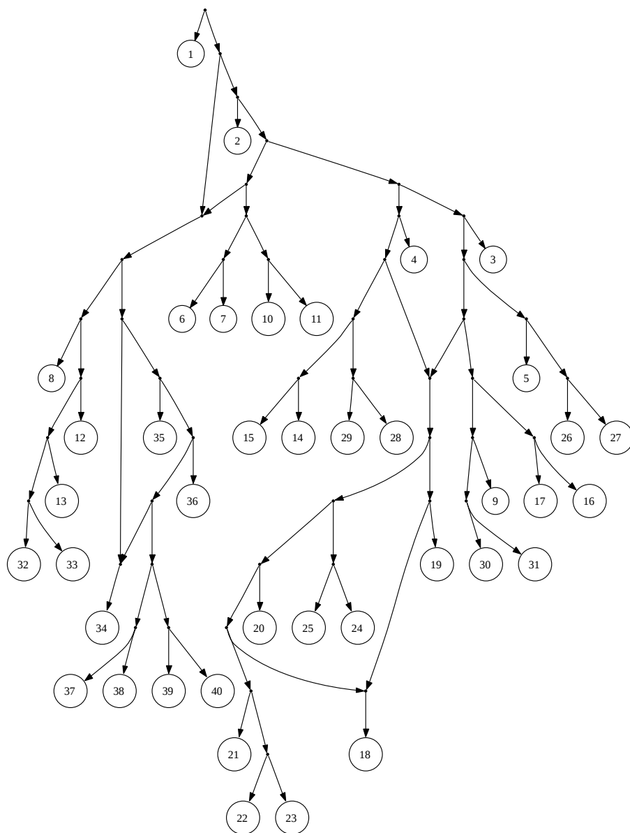
Figure 4.28: The network constructed by MARLON for the simulated triplet set T^* .
